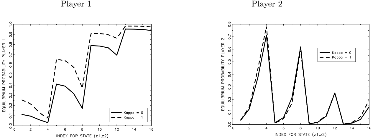
Figure 3: Equilibrium Probabilities
